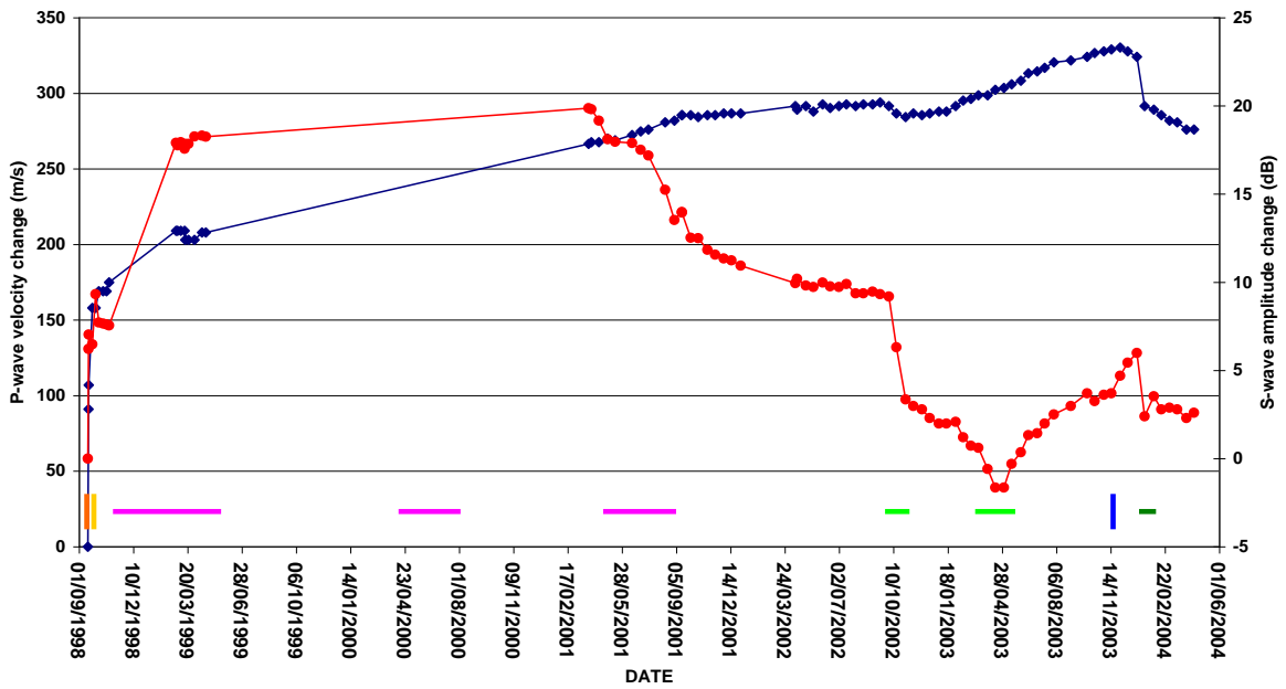
Figure 5: P-wave velocity and amplitude for a ray-path through the concrete bulkhead over a 5-year period of the TSX. (Blue = P-wave, red = S-wave)
