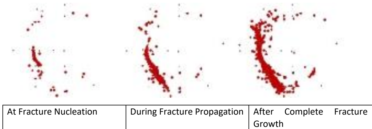
Figure 6: Located AE events at 3 different stages through the curing stage of the TSX (16th September - 27th October 1998).
